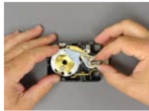
Slide the short bolt into the lock case while holding down the relock trigger arm. Re-install the lever screw, being careful to move the lever as little as possible.
