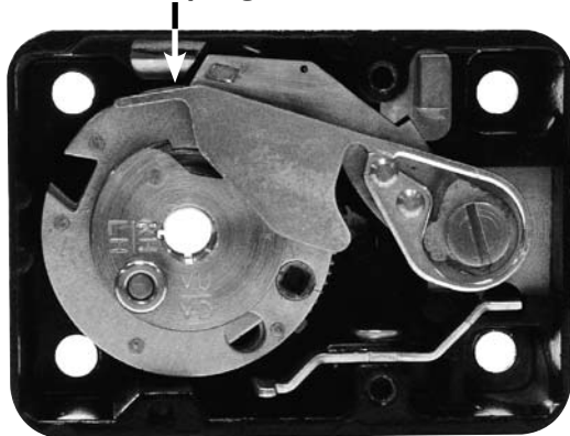
Accelerator Spring in Released Position
