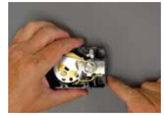
Tighten the lever screw firmly, using either the change key rib or a large flat-tip screwdriver.
