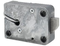
6106 Pivot bolt lock housed within the safe. Provides for Bank and Service modes of operation
