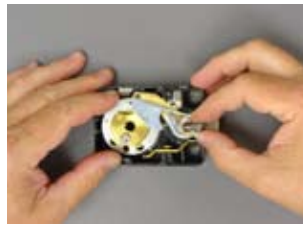
Slide the short bolt into the lock case while holding down the reload trigger arm. Re-install the lever screw, being careful to move the lever as little as possible.
